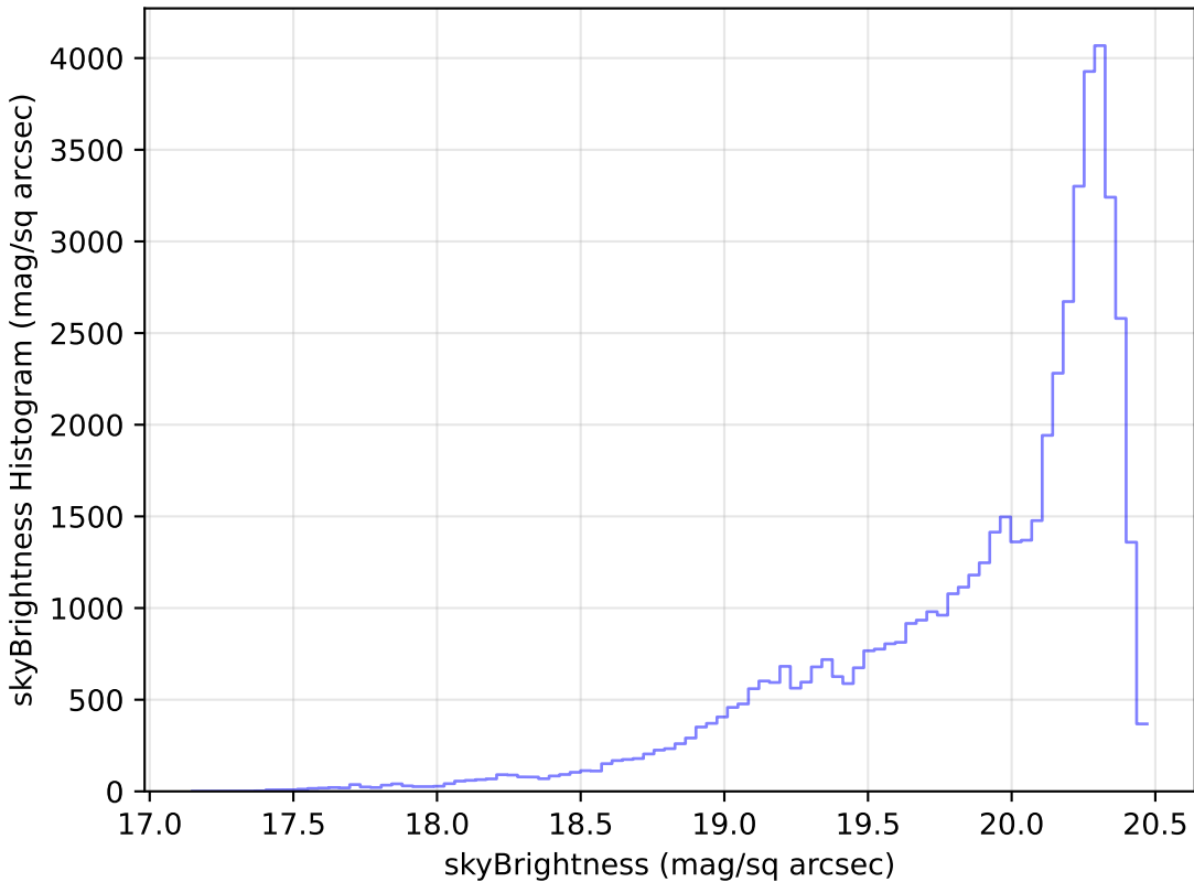
ddf_loaded_fl8_v3.4_10yrs Yr 1 i band: skyBrightness Histogram
