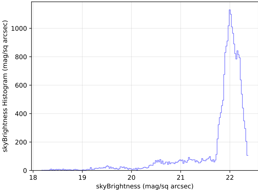
ddf_loaded_fl8_v3.4_10yrs Yr 1 g band: skyBrightness Histogram
