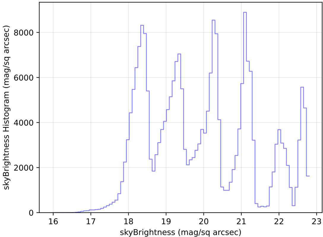
ddf_loaded_fl8_v3.4_10yrs Yr 1 all bands: skyBrightness Histogram
