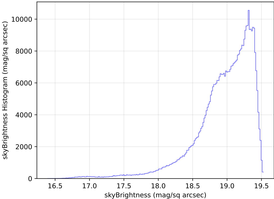
ddf_loaded_fl8_v3.4_10yrs WFD z band: skyBrightness Histogram
