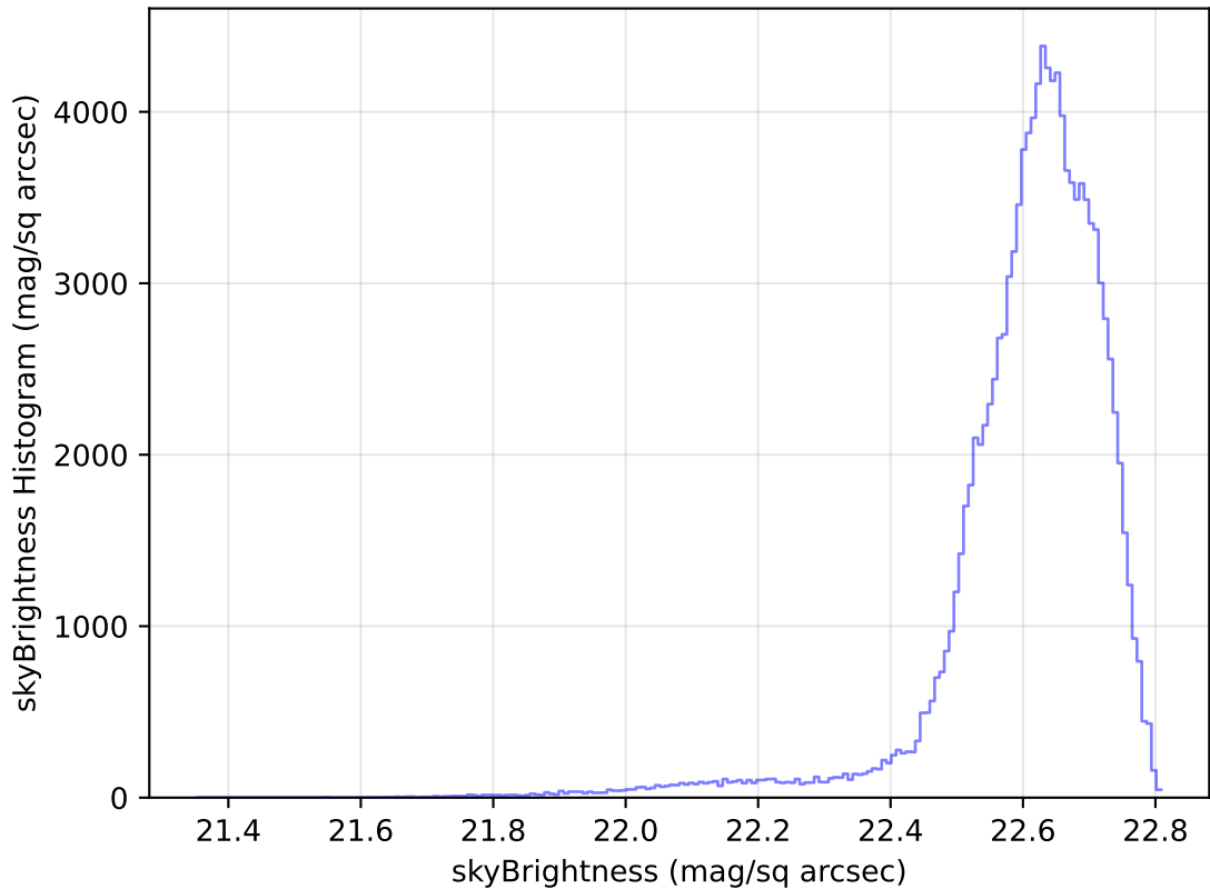
ddf_loaded_fl8_v3.4_10yrs WFD u band: skyBrightness Histogram
