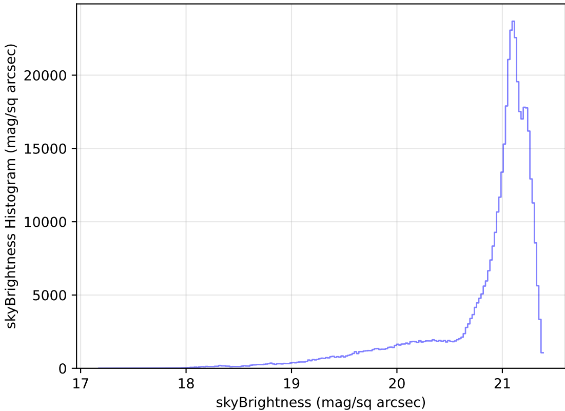
ddf_loaded_fl8_v3.4_10yrs WFD r band: skyBrightness Histogram
