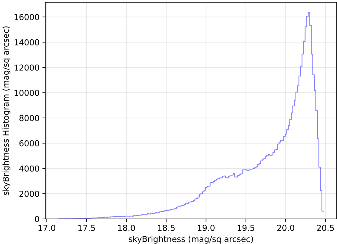
ddf_loaded_fl8_v3.4_10yrs WFD i band: skyBrightness Histogram
