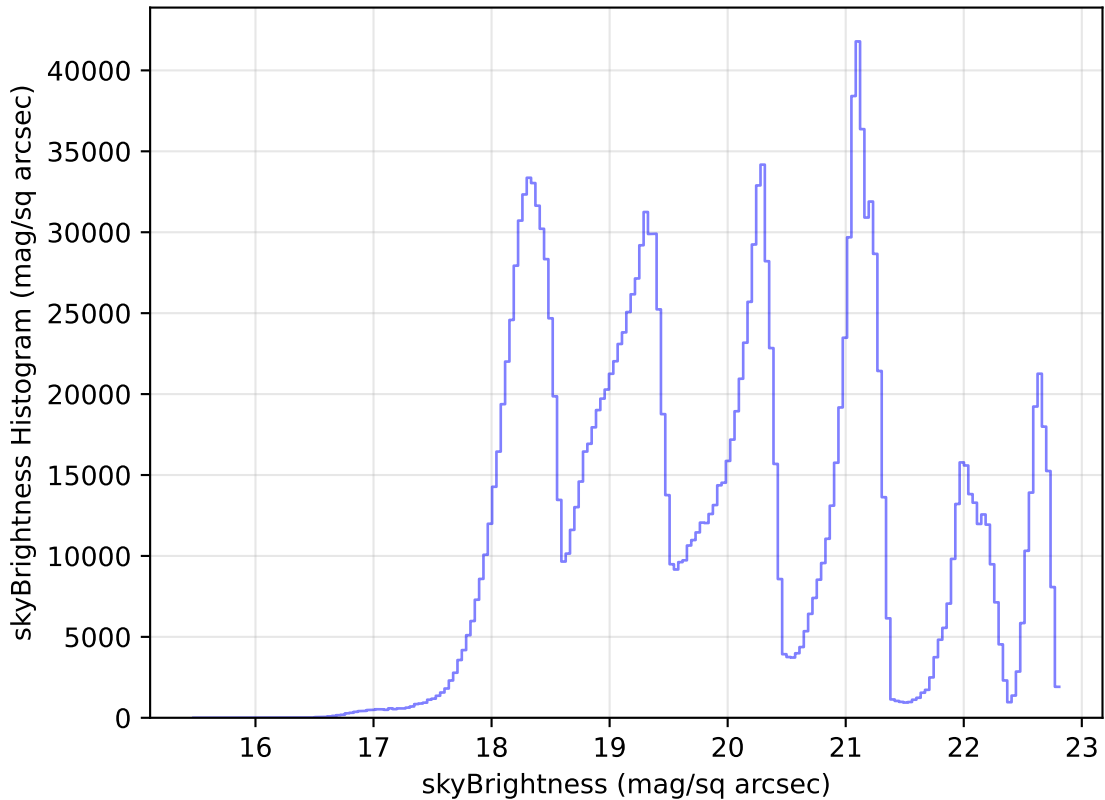
ddf_loaded_fl8_v3.4_10yrs WFD all bands: skyBrightness Histogram
