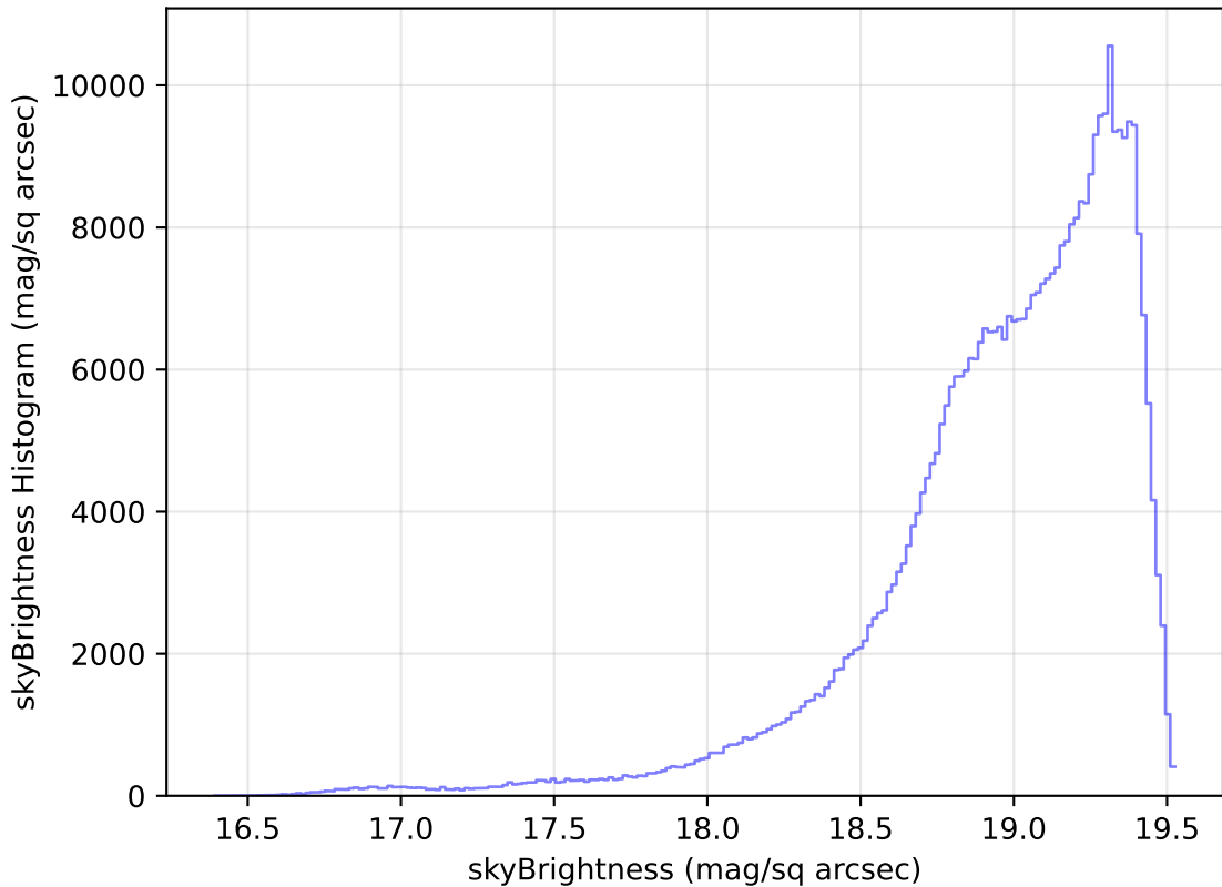
ddf_loaded_fl8_v3.4_10yrs All sky z band: skyBrightness Histogram
