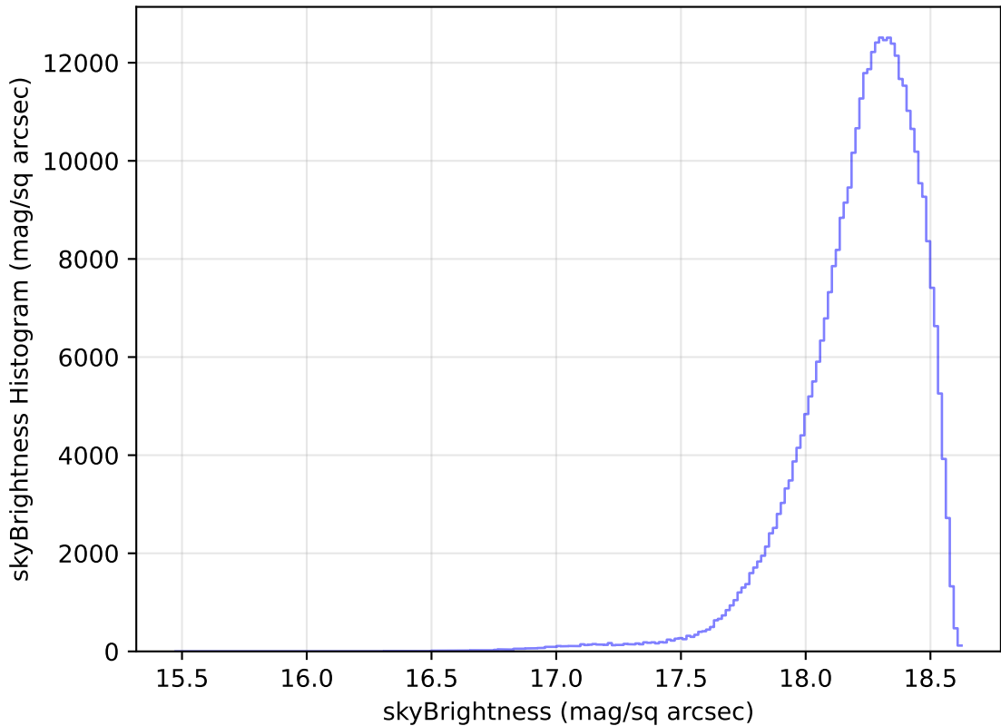
ddf_loaded_fl8_v3.4_10yrs All sky y band: skyBrightness Histogram
