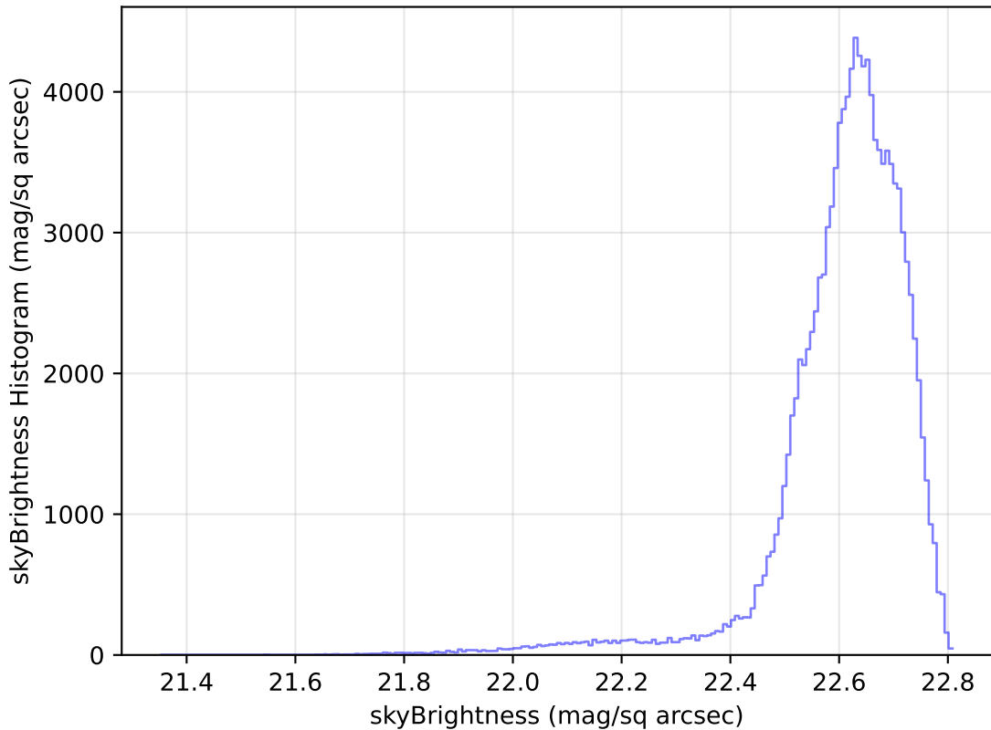
ddf_loaded_fl8_v3.4_10yrs All sky u band: skyBrightness Histogram
