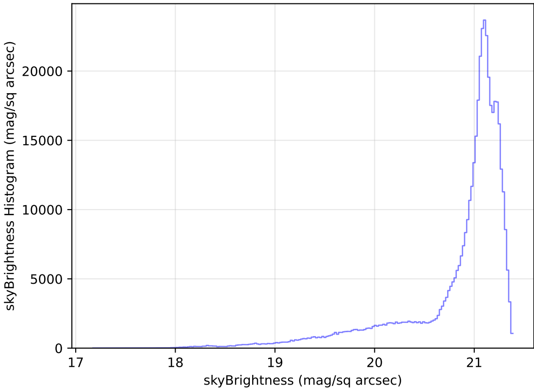
ddf_loaded_fl8_v3.4_10yrs All sky r band: skyBrightness Histogram
