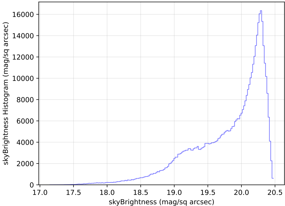
ddf_loaded_fl8_v3.4_10yrs All sky i band: skyBrightness Histogram
