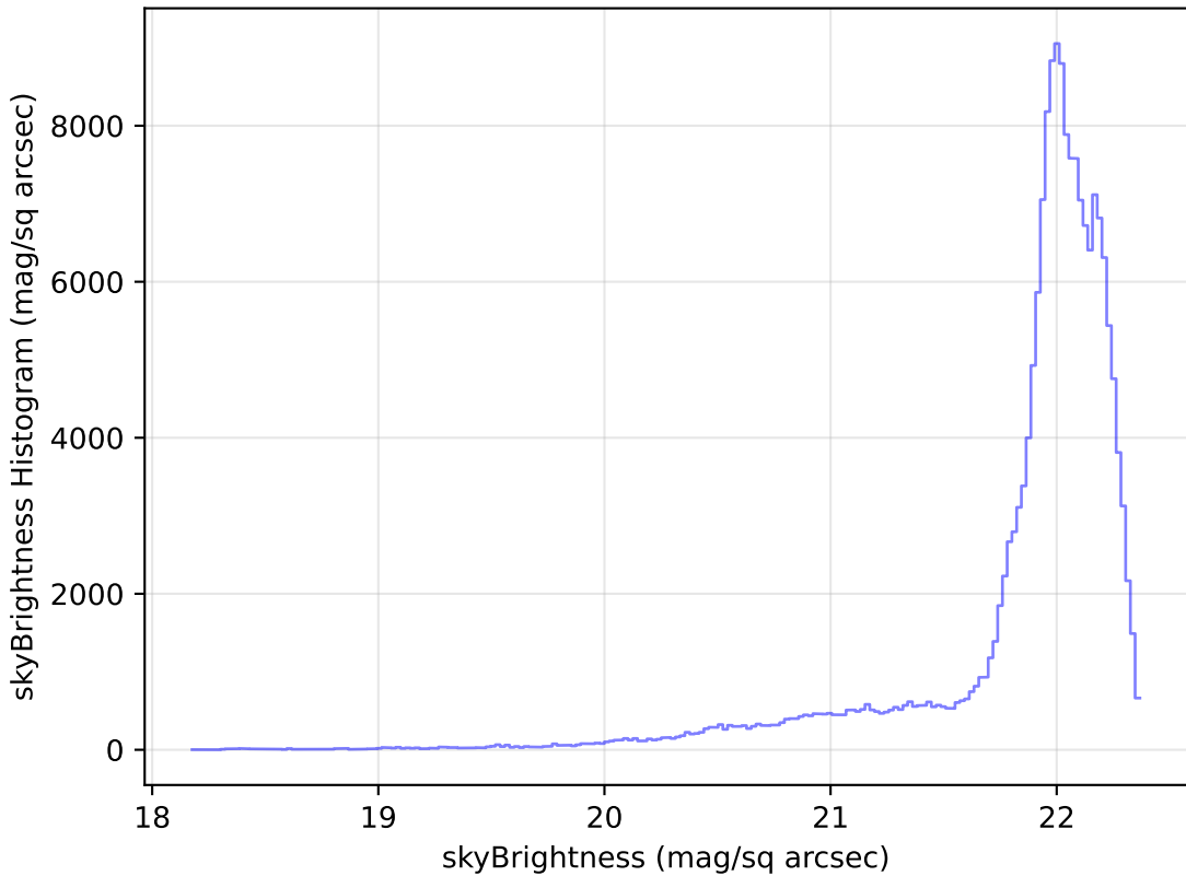
ddf_loaded_fl8_v3.4_10yrs All sky g band: skyBrightness Histogram
