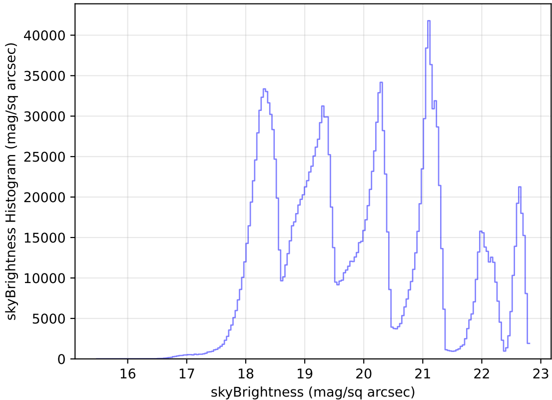
ddf_loaded_fl8_v3.4_10yrs All sky all bands: skyBrightness Histogram
