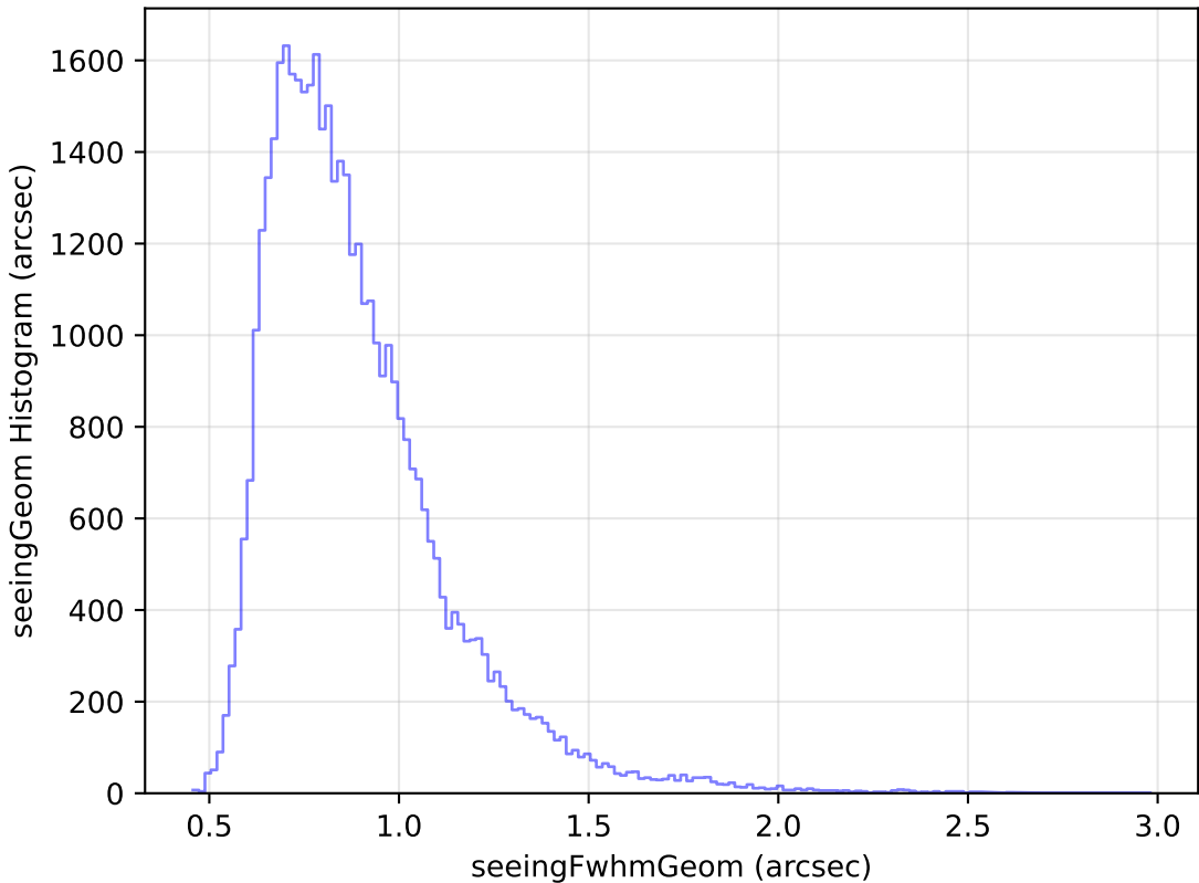
ddf_loaded_fl8_v3.4_10yrs Yr 1 z band: seeingGeom Histogram
