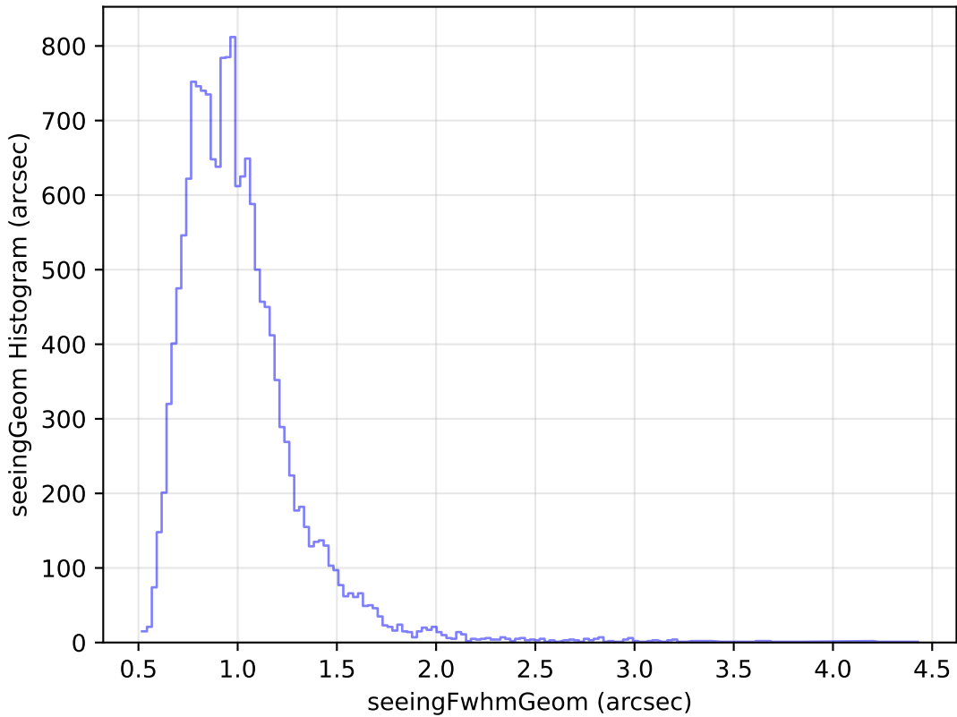
ddf_loaded_fl8_v3.4_10yrs Yr 1 u band: seeingGeom Histogram
