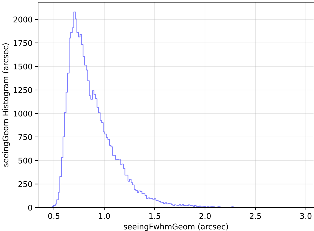
ddf_loaded_fl8_v3.4_10yrs Yr 1 r band: seeingGeom Histogram
