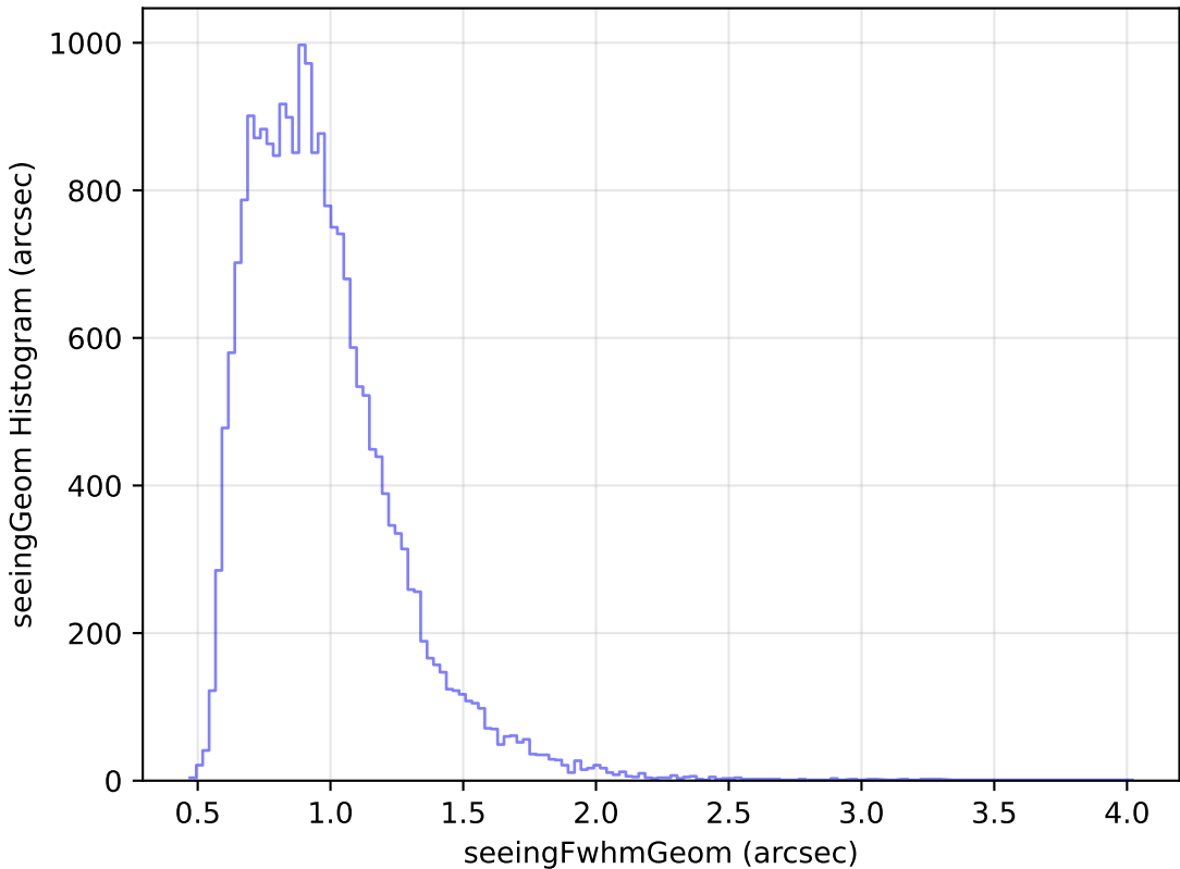
ddf_loaded_fl8_v3.4_10yrs Yr 1 g band: seeingGeom Histogram
