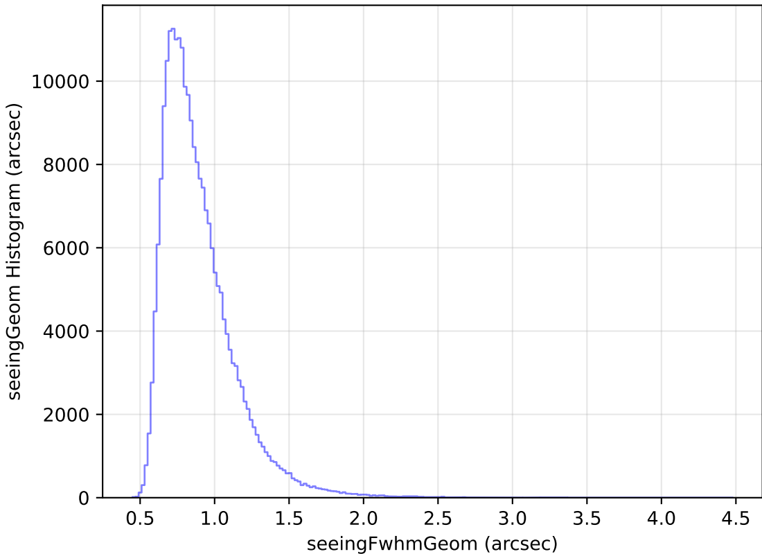
ddf_loaded_fl8_v3.4_10yrs Yr 1 all bands: seeingGeom Histogram
