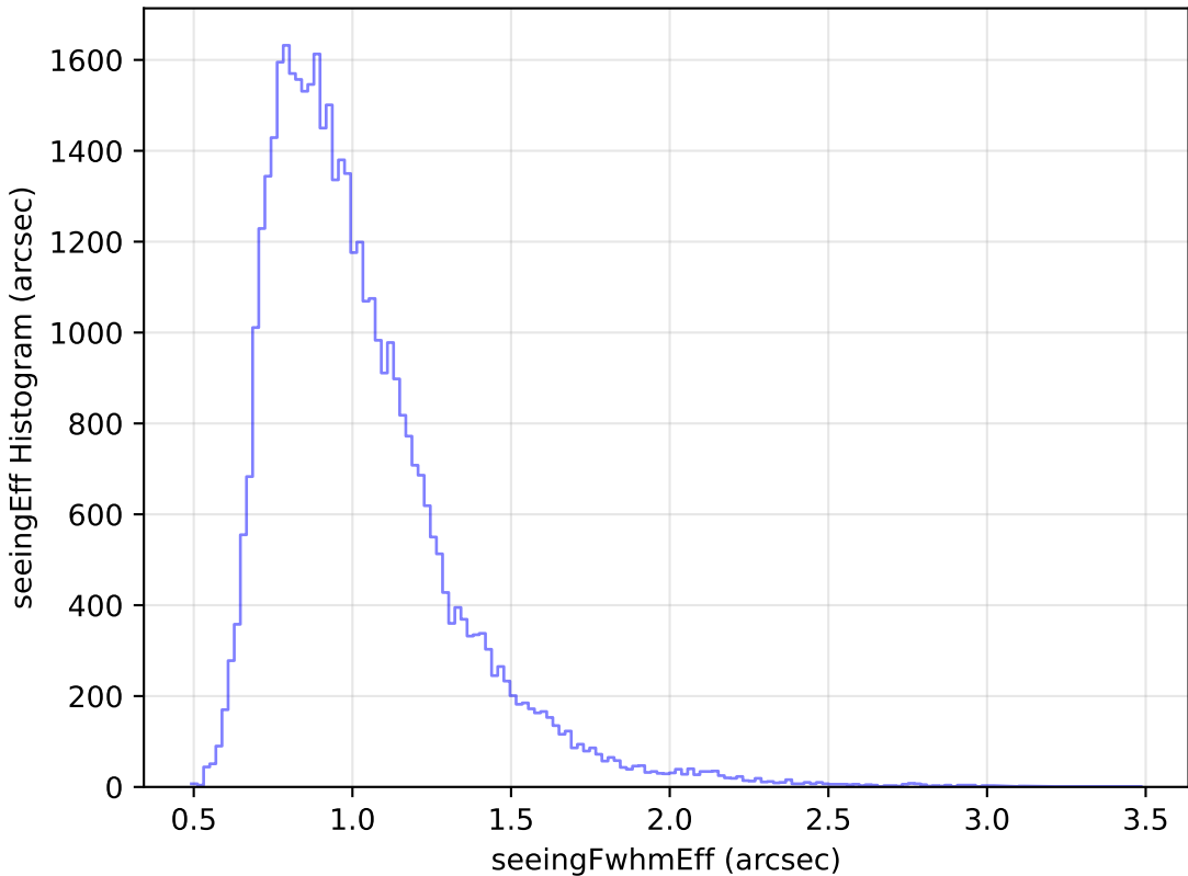
ddf_loaded_fl8_v3.4_10yrs Yr 1 z band: seeingEff Histogram
