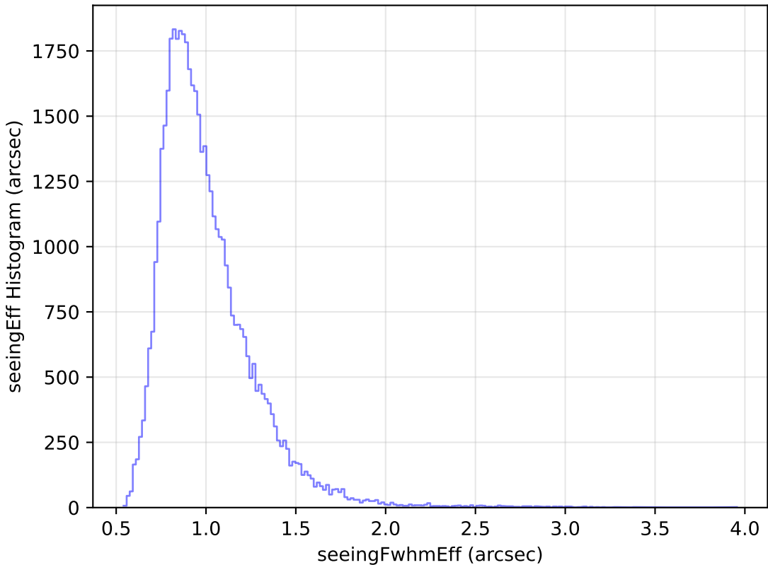
ddf_loaded_fl8_v3.4_10yrs Yr 1 y band: seeingEff Histogram
