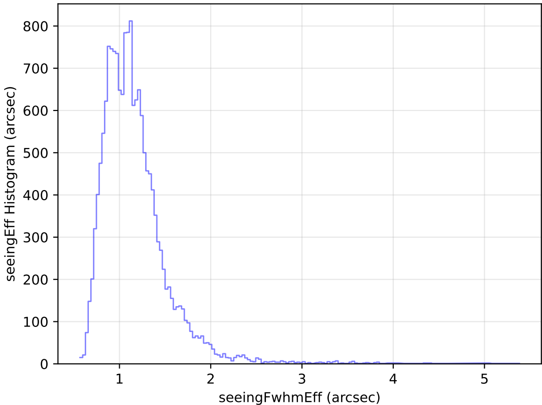
ddf_loaded_fl8_v3.4_10yrs Yr 1 u band: seeingEff Histogram
