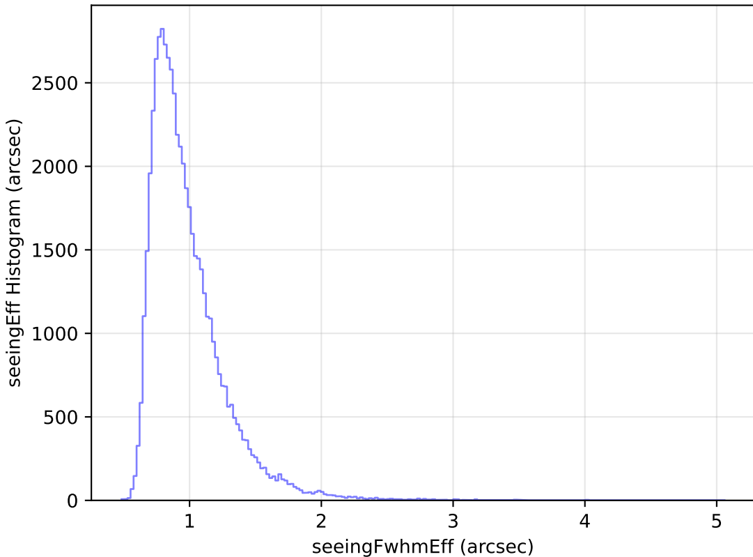
ddf_loaded_fl8_v3.4_10yrs Yr 1 i band: seeingEff Histogram
