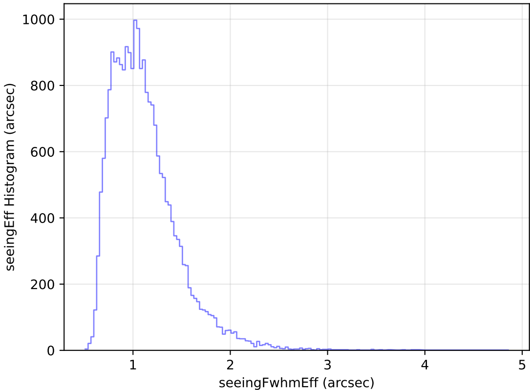
ddf_loaded_fl8_v3.4_10yrs Yr 1 g band: seeingEff Histogram
