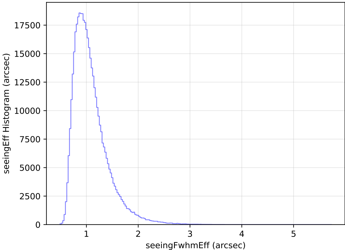
ddf_loaded_fl8_v3.4_10yrs WFD z band: seeingEff Histogram
