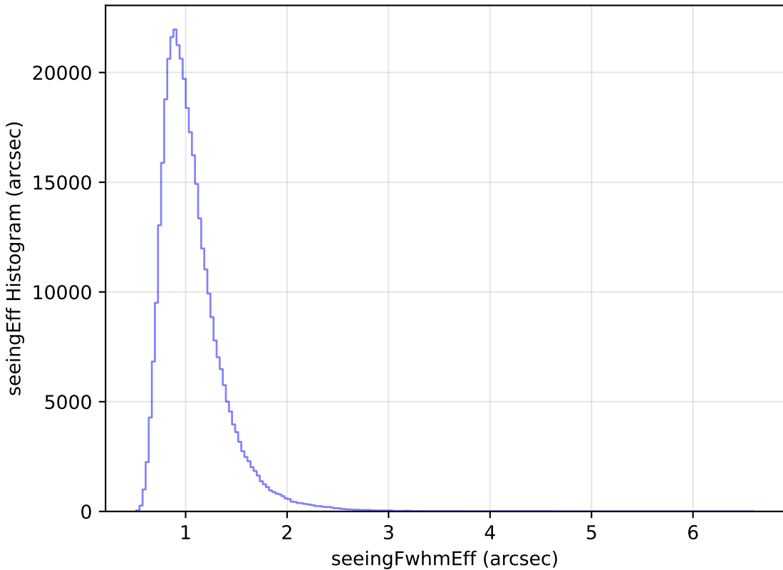
ddf_loaded_fl8_v3.4_10yrs WFD y band: seeingEff Histogram
