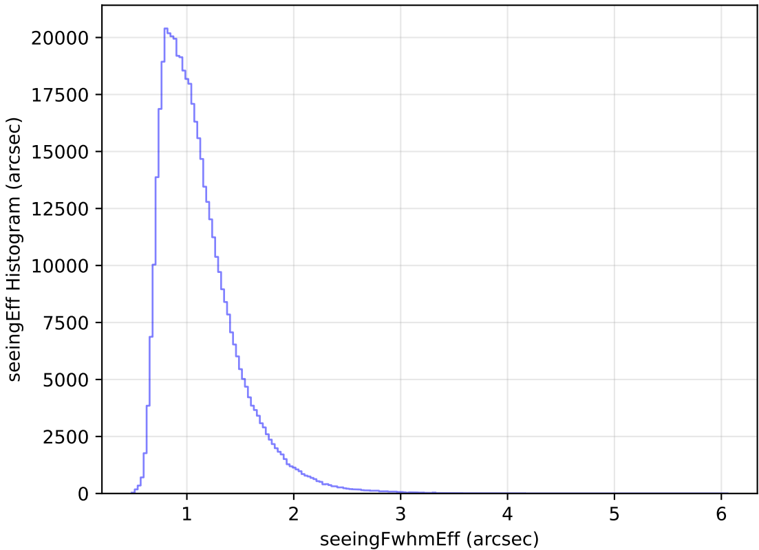
ddf_loaded_fl8_v3.4_10yrs WFD r band: seeingEff Histogram
