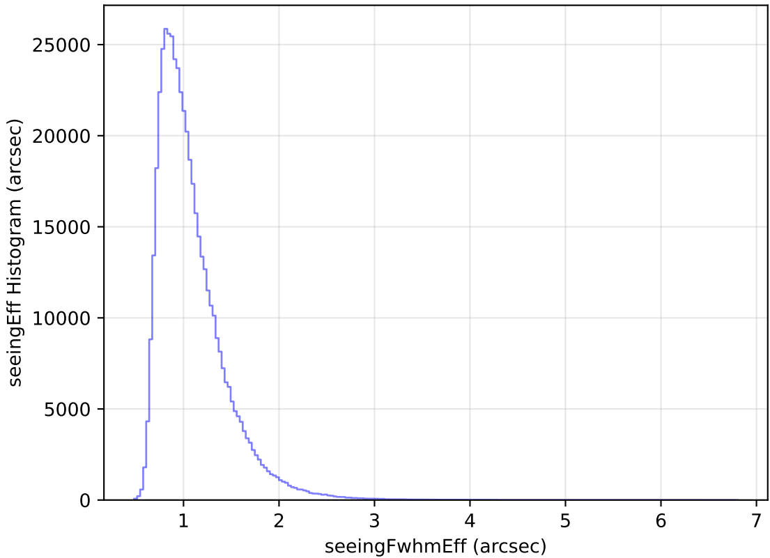
ddf_loaded_fl8_v3.4_10yrs WFD i band: seeingEff Histogram
