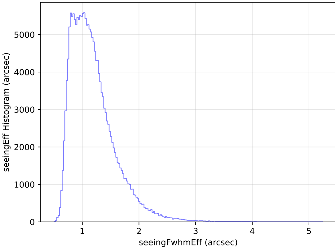
ddf_loaded_fl8_v3.4_10yrs WFD g band: seeingEff Histogram
