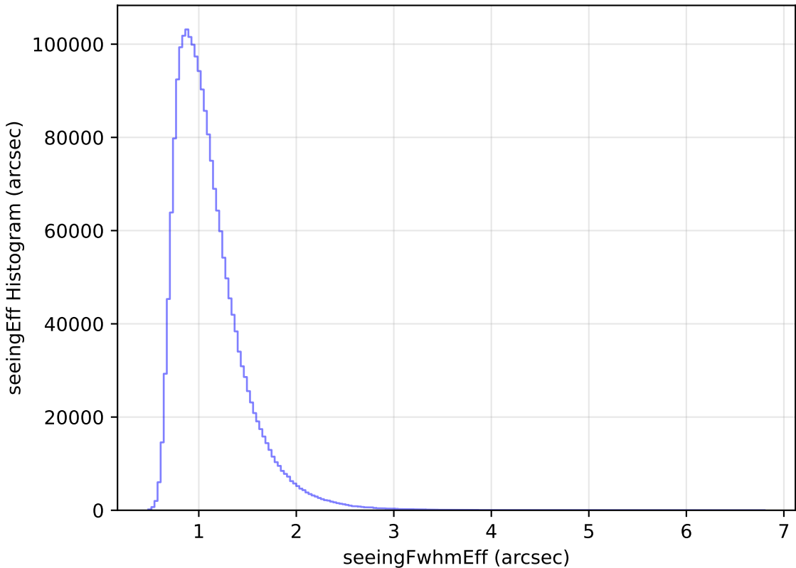
ddf_loaded_fl8_v3.4_10yrs WFD all bands: seeingEff Histogram
