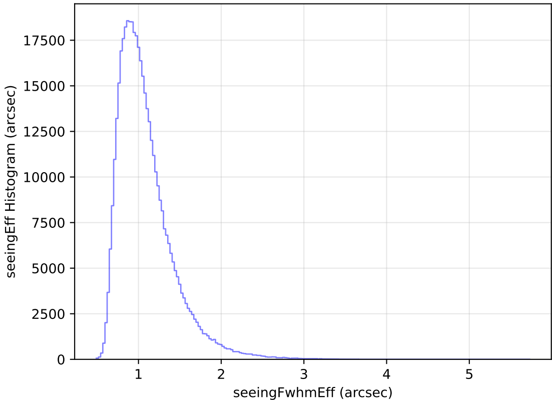
ddf_loaded_fl8_v3.4_10yrs All sky z band: seeingEff Histogram
