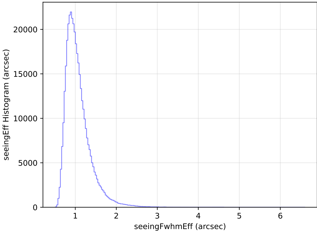
ddf_loaded_fl8_v3.4_10yrs All sky y band: seeingEff Histogram
