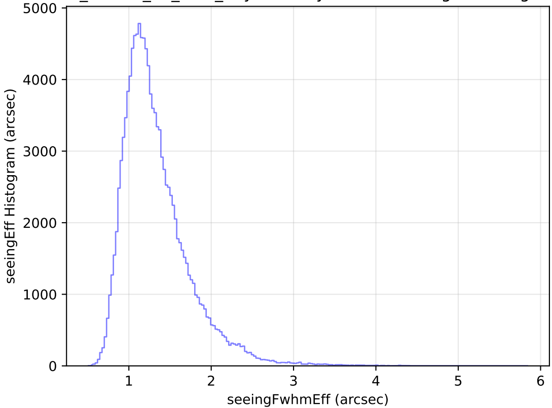
ddf_loaded_fl8_v3.4_10yrs All sky u band: seeingEff Histogram
