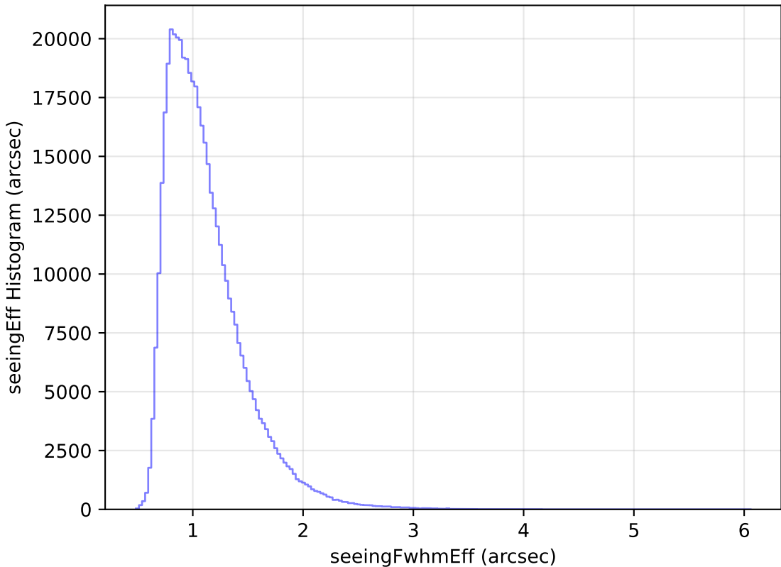
ddf_loaded_fl8_v3.4_10yrs All sky r band: seeingEff Histogram
