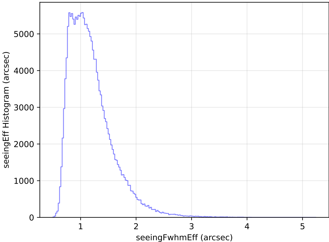
ddf_loaded_fl8_v3.4_10yrs All sky g band: seeingEff Histogram
