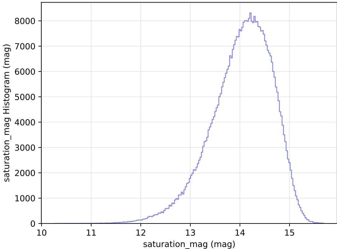
ddf_loaded_fl8_v3.4_10yrs WFD z band: saturation_mag Histogram
