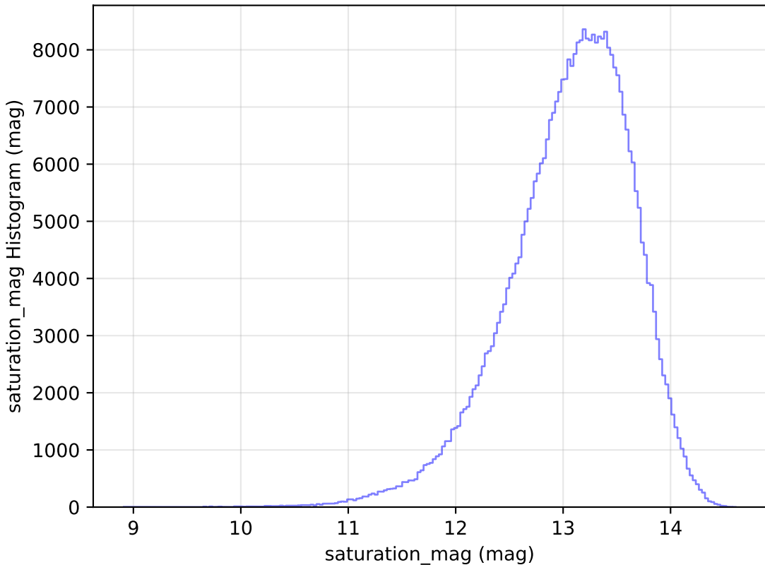
ddf_loaded_fl8_v3.4_10yrs WFD y band: saturation_mag Histogram
