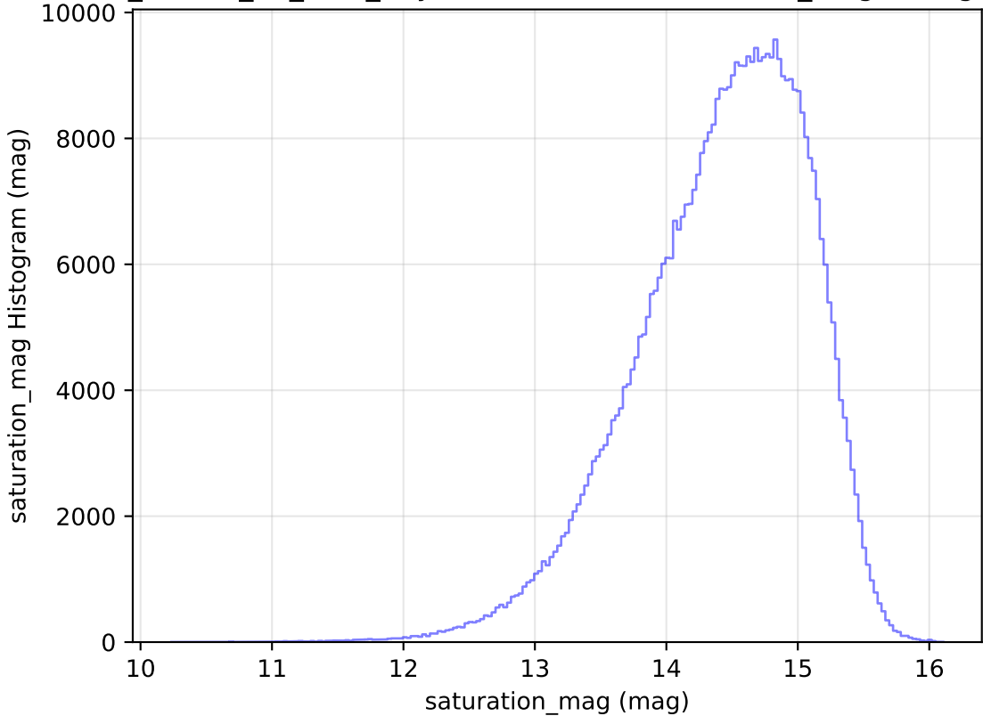
ddf_loaded_fl8_v3.4_10yrs WFD i band: saturation_mag Histogram
