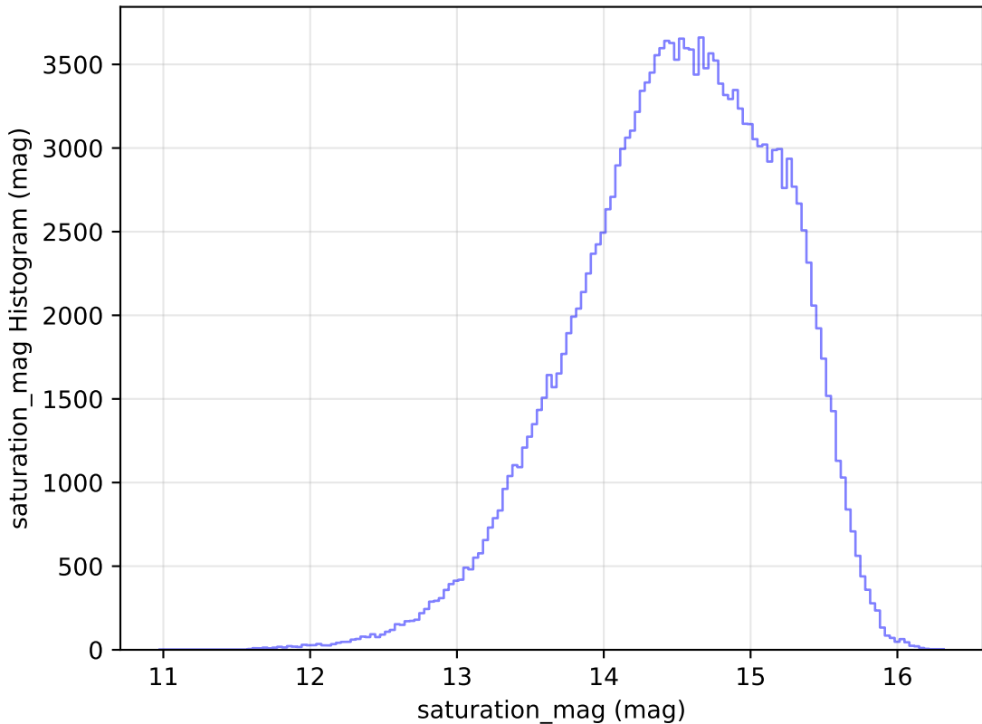
ddf_loaded_fl8_v3.4_10yrs WFD g band: saturation_mag Histogram
