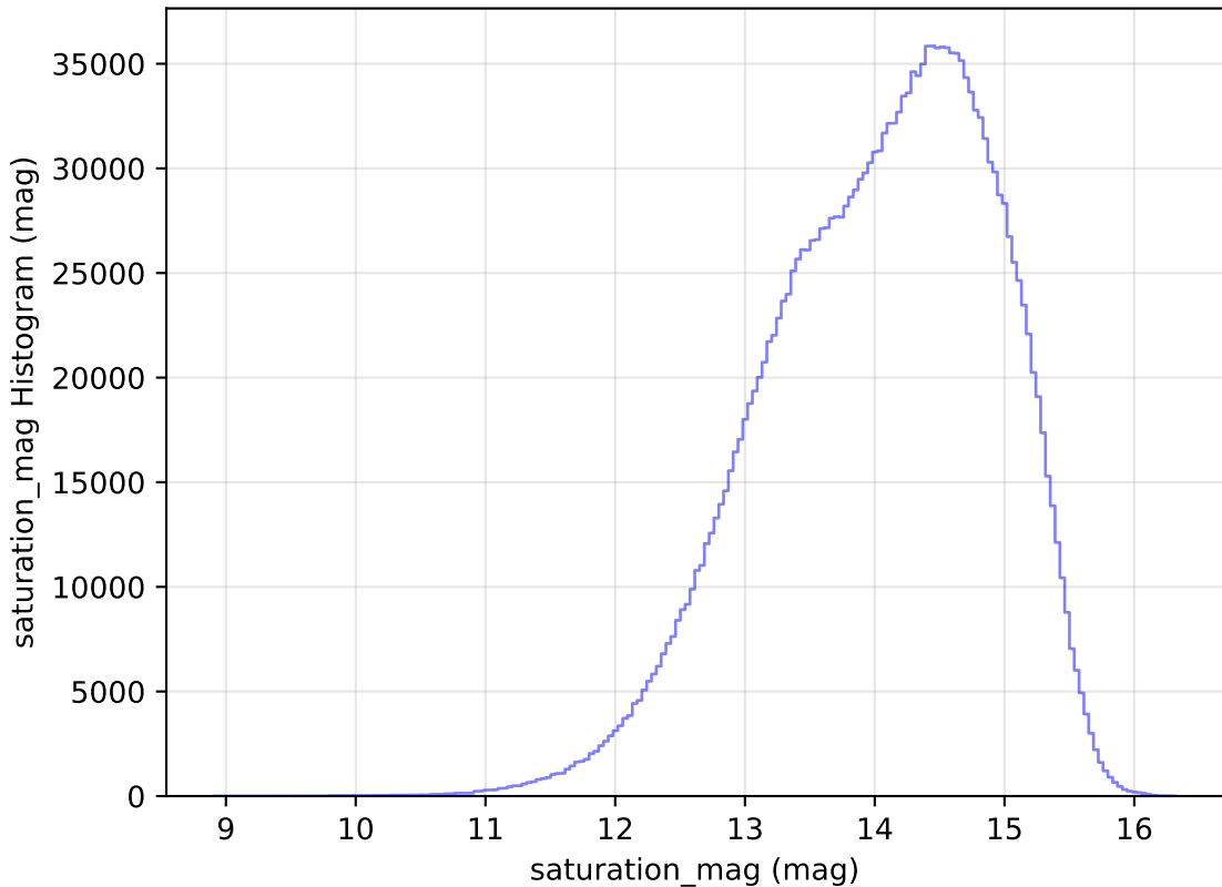
ddf_loaded_fl8_v3.4_10yrs WFD all bands: saturation_mag Histogram
