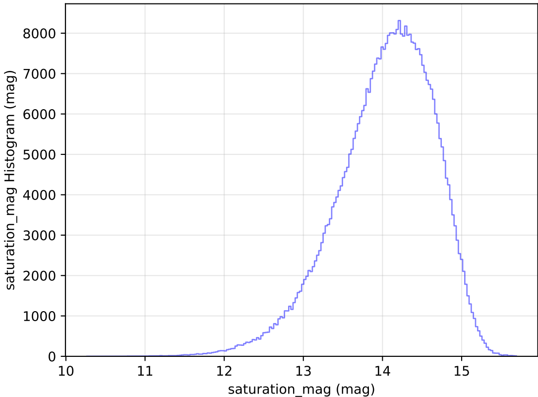
ddf_loaded_fl8_v3.4_10yrs All sky z band: saturation_mag Histogram
