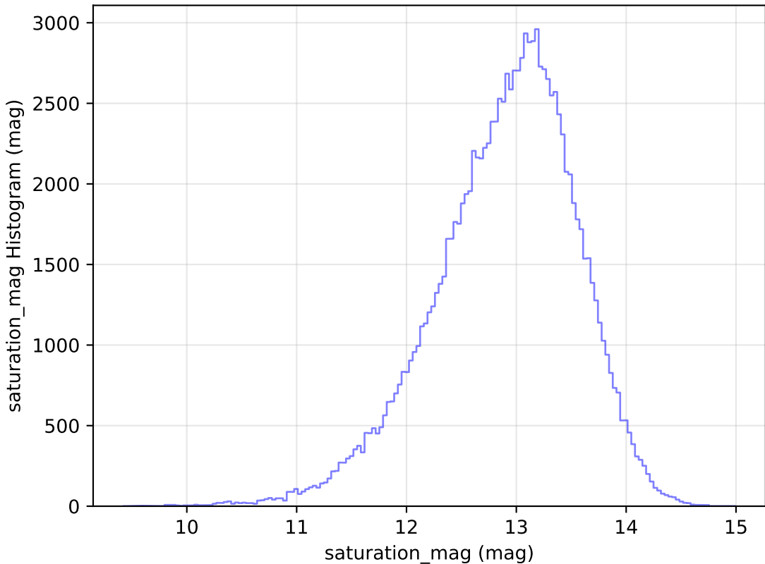
ddf_loaded_fl8_v3.4_10yrs All sky u band: saturation_mag Histogram
