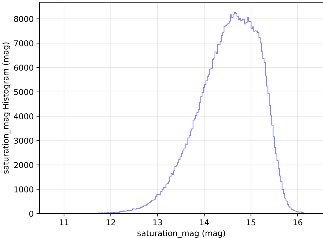
ddf_loaded_fl8_v3.4_10yrs All sky r band: saturation_mag Histogram
