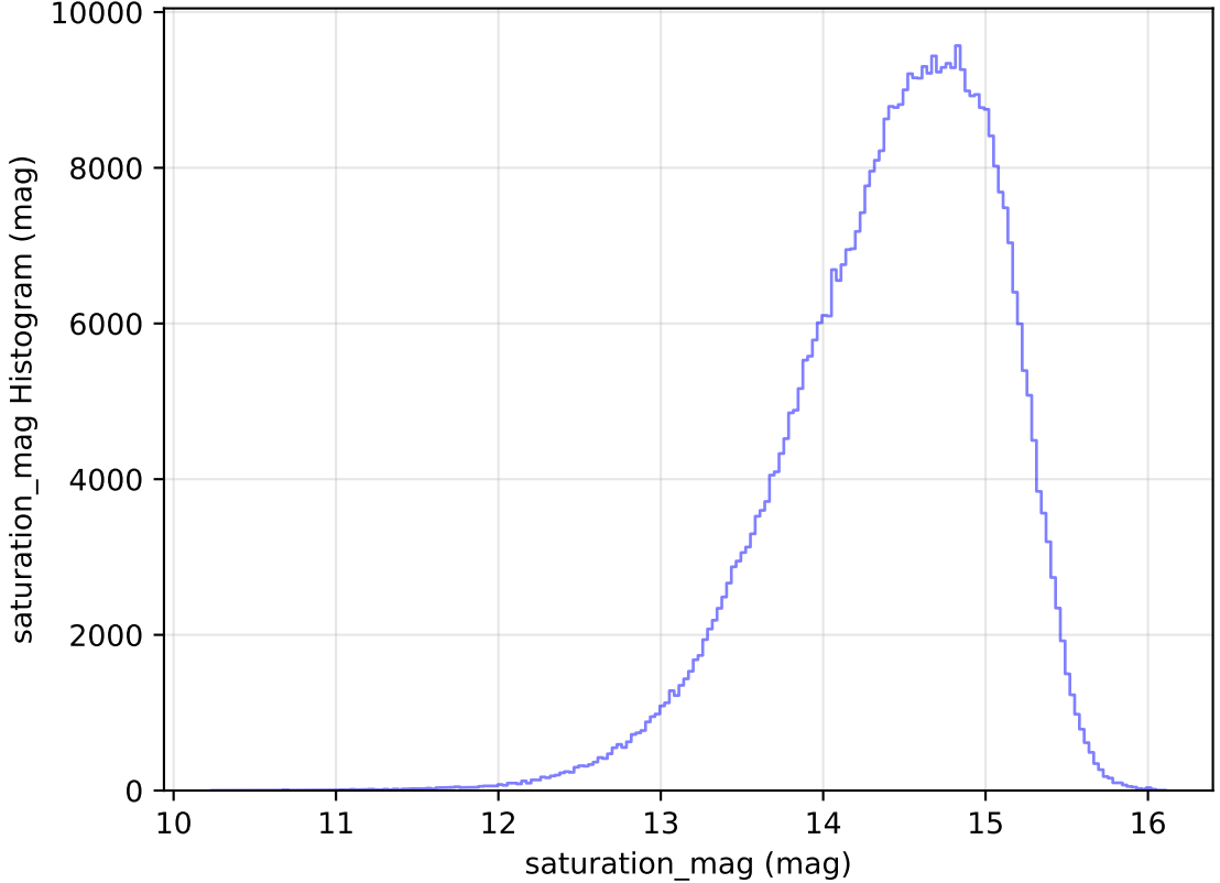
ddf_loaded_fl8_v3.4_10yrs All sky i band: saturation_mag Histogram
