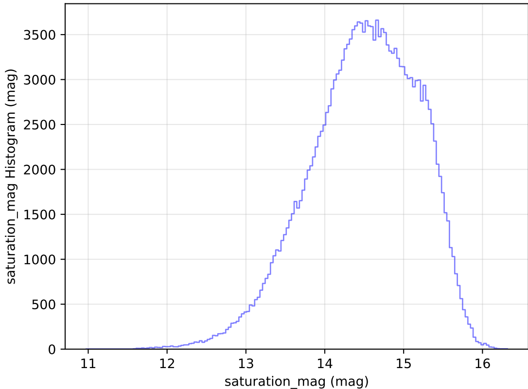
ddf_loaded_fl8_v3.4_10yrs All sky g band: saturation_mag Histogram
