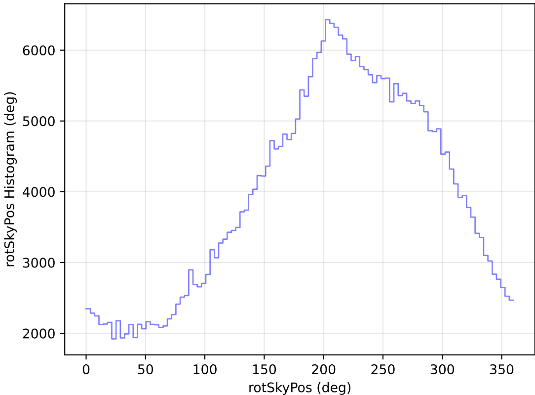
ddf_loaded_fl8_v3.4_10yrs WFD y band: rotSkyPos Histogram
