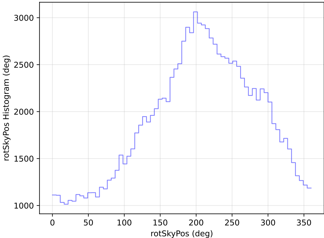
ddf_loaded_fl8_v3.4_10yrs WFD u band: rotSkyPos Histogram
