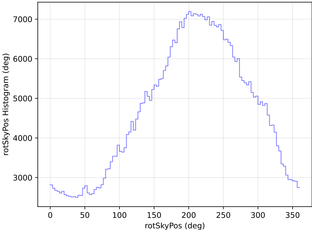
ddf_loaded_fl8_v3.4_10yrs WFD i band: rotSkyPos Histogram
