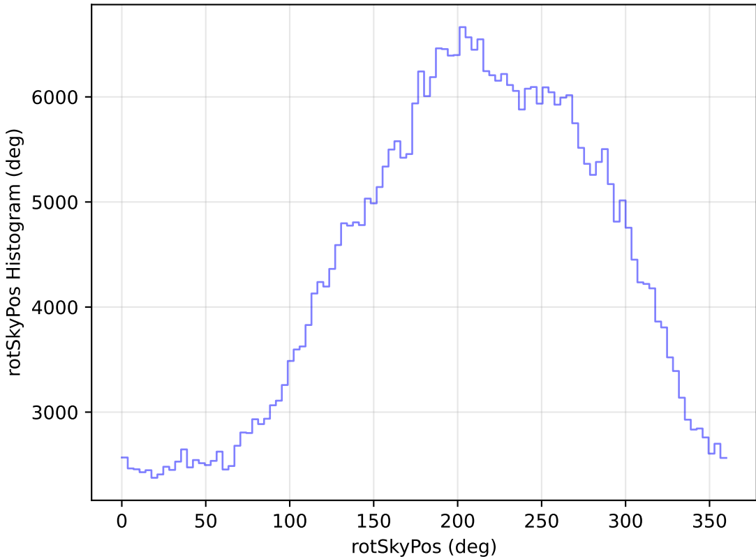
ddf_loaded_fl8_v3.4_10yrs All sky z band: rotSkyPos Histogram
